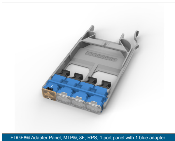
EDGE8® Adapter Panel, MTP®, 8F, RPS, 1 port panel with 1 blue adapter
